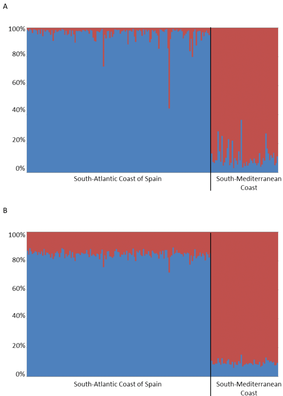
Figure 1 Clustering analysis in STRUCTURE considering information about population of origin ( k = 2 ). Individuals are represented as vertical bars, where the amount of each colour indicates the proportion of each inferred cluster. A represents the clusters obtained in the simulations considering the absence of null alleles while B represents those assuming them. Isla Canela and Doñana are represented by the label “South-Atlantic Coast of Spain”, and Caleta de Vélez by the label “South-Mediterranean Coast”.
